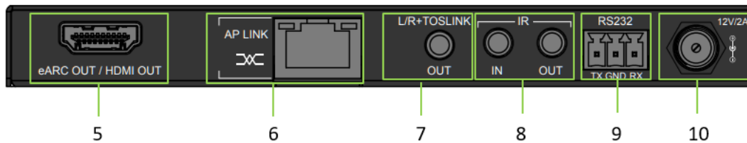
AC-AEX-DEARC-R (Receiver) – Rear Panel
